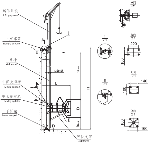
III型安装
