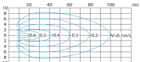
MA10/12-620-480
