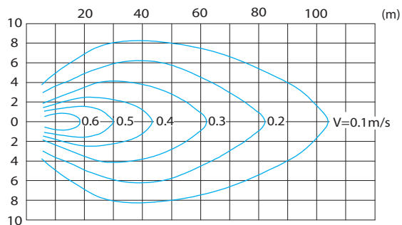
MA15/12-620-480
